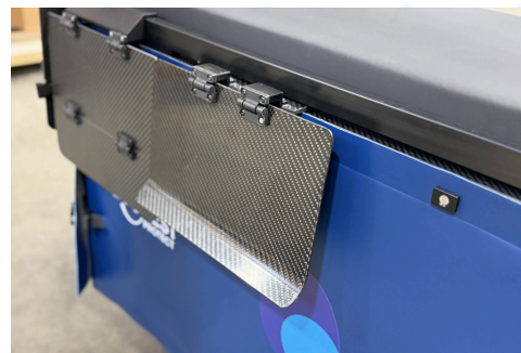
Figure 31: Side Flip Shield articulation
